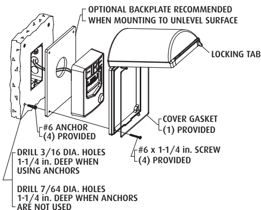
Fig. 3 - FLUSH MOUNTING OPTION
