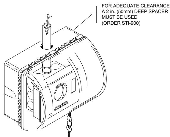
FOR SURFACE MOUNT STI-9110 AND STI-900
