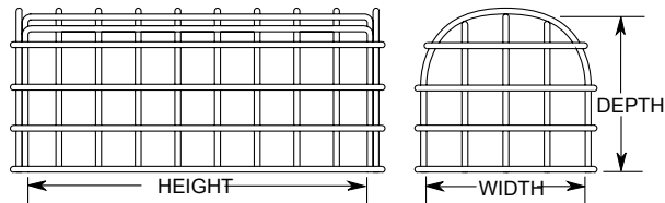
STI-9621/9622 SIDE VIEW STI-9621/9622 END VIEW
